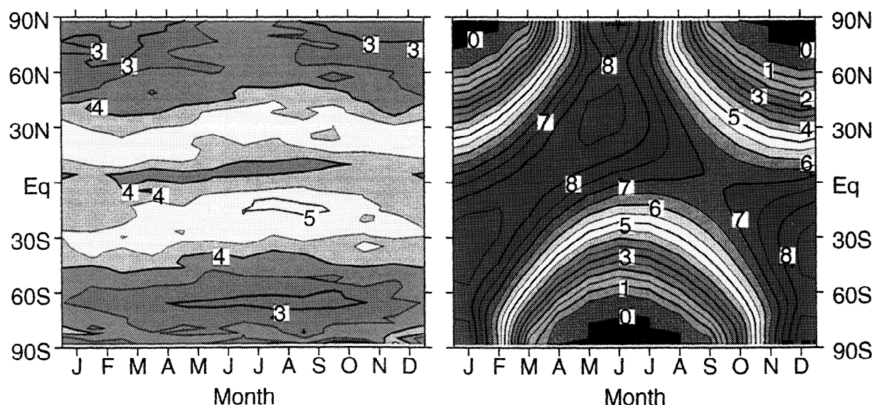
Plate 1. Change in net longwave radiative flux at the tropopause when \text{CO}_2 is doubled (left panel) with respect to the control case and the reduction in incoming solar radiation (right panel) needed to compensate this forcing. Both values ( \text{W m}^{-2} ) are zonally averaged as a function of time of year. Change in solar radiation has a latitudinal and seasonal pattern markedly different from the radiative forcing of \text{CO}_2 .
