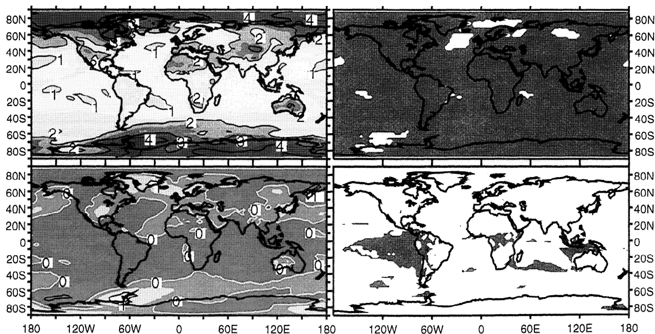
Plate 2. Surface temperature changes (left panels) and areas with changes that are statistically significant at the 5% level (right panels) for the Doubled- \text{CO}_2 (top panels) and the Geoengineered (bottom panels) simulations. Solar radiation has a spatial pattern that differs greatly from that of radiative forcing due to doubling atmospheric \text{CO}_2 content, yet a reduction in solar forcing largely compensates the temperature response to \text{CO}_2 -doubling.
